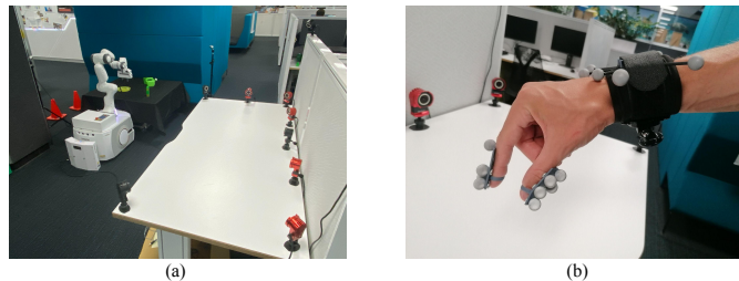
Fig. 1: (a) Motion capture and robot setup. (b) The robot was teleoperated by a human operator equipped with a motion capture system for hand gestures and movements detection.
